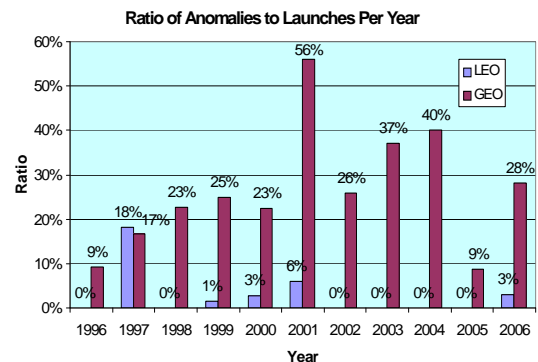
Figure 5: Ratio of anomalies by year by orbit
