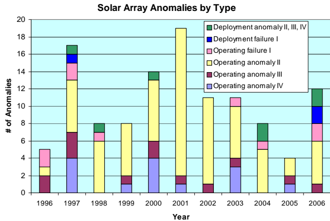
Figure 2: Solar Array Anomalies by Type
