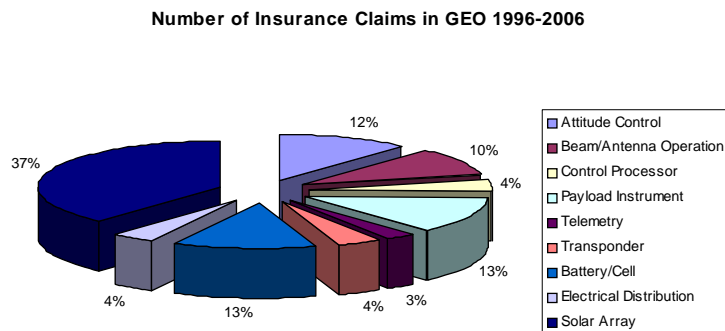
Figure 7: Number of Insurance Claims in GEO in last ten years
