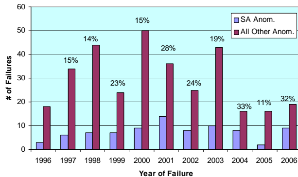
Figure 1: Solar array anomalies vs. all anomalies in GEO
